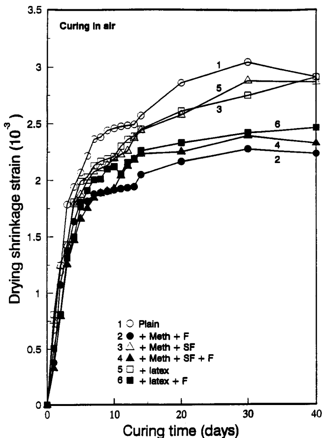
Fig. 2 Drying shrinkage strain vs. curing time. Meth = methylcellulose; SF = silica fume; F = fibers.
